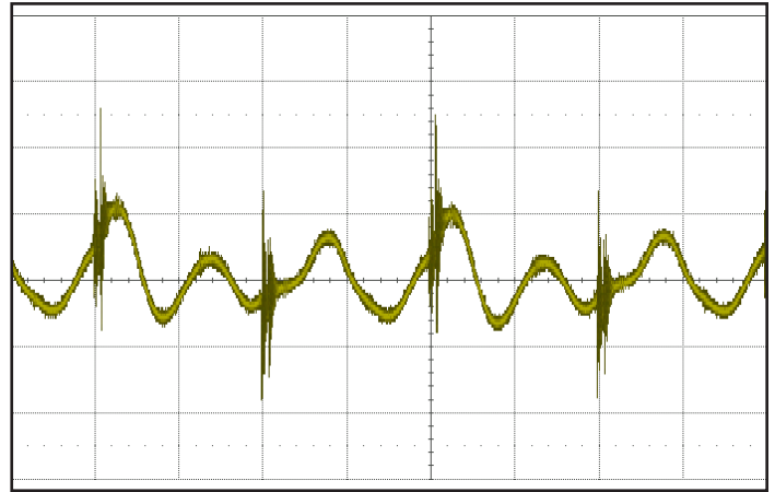
Figure 14: Output voltage ripple at nominal input voltage and rated load current (50 mV/div, 2 \mu s/div). Load capacitance: 1 \mu F ceramic capacitor and 15 \mu F tantalum capacitor. Bandwidth: 20 MHz. See Figure 11.
