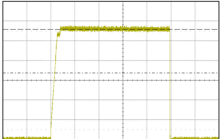
Figure 16: Load current (10A/div; 10ms/div) as a function of time when the converter attempts to turn on into a 1 mW short circuit.
