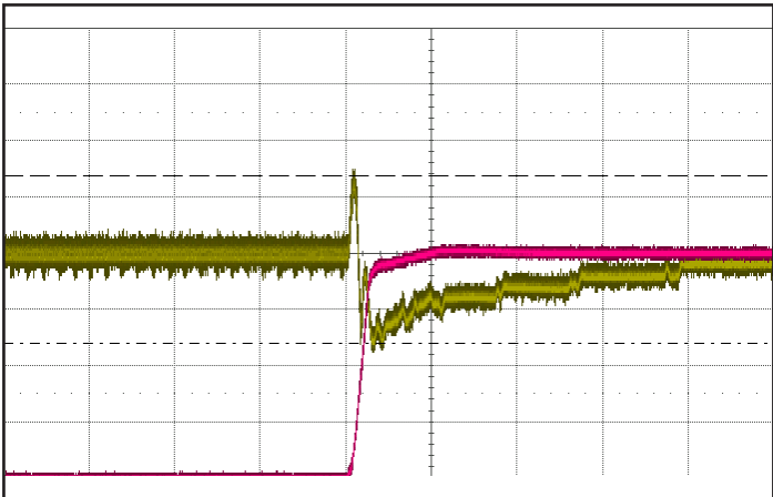
Figure 15: Output voltage response to step-change in input voltage (35V to 75V in 300 \mu s, 1 ms/div). Load cap: 470 \mu F, 15mW ESR electrolytic capacitor. Ch 1: V_{out} (500mV/div), Ch 2: V_{in} (10V/div), at zero load current.
