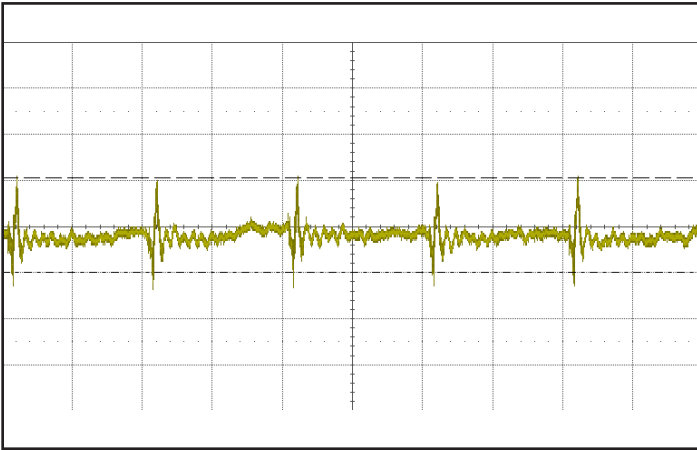
Figure 13: Input reflected ripple current, is, through a 4.7 \mu H source inductor, using a 220 \mu F input capacitor, at nominal input voltage and rated load current (10 mA/div, 2 \mu s/div). See Figure 11.
