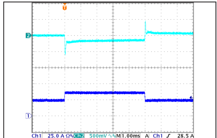
Figure 10: Output voltage response to step-change in load current [50%-75%-50% of I_{out(max)} ; dI/dt = 5A/\mu s ]. Load cap: 470\mu F , 15mW ESR electrolytic capacitor. Top trace: Vout (500mV/div), Bottom trace: Iout (25A/div).
