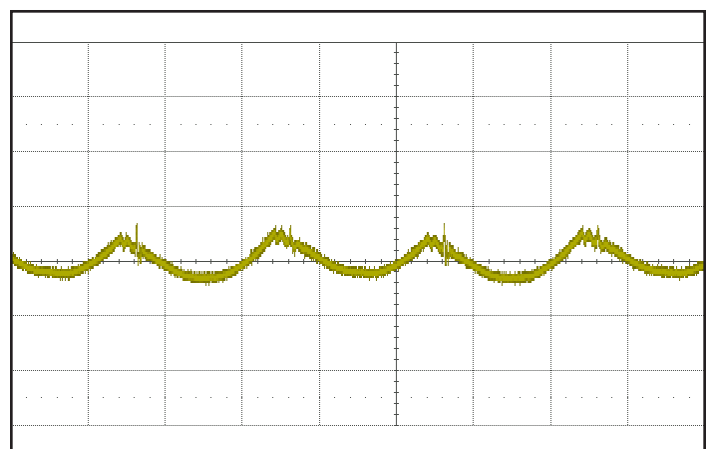
Figure 12: Input Terminal Ripple Current, i_c , at full rated output current and nominal input voltage with 4.7\mu H source impedance and 220\mu F electrolytic capacitor (1 A/div, 2\mu s/div ). See Figure 11.
