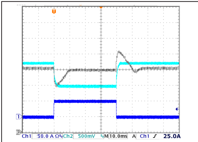
Figure D: Output voltage response to full load step change in output current (Ch2), compared to a fully regulated HZA model (Ref2). 12mF output capacitance.
