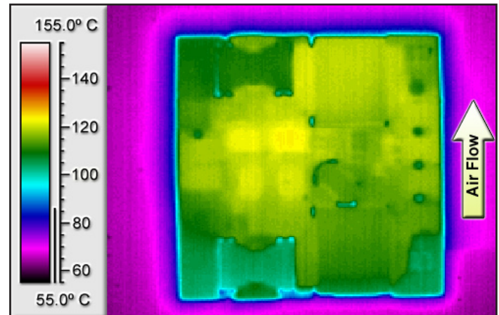
Figure 4: Thermal plot of converter at 36A load current (432W) with 55°C air flowing at the rate of 200 LFM. Air is flowing across the converter from pin 5 to pin 9 (nominal input voltage).
