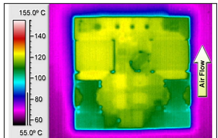
Figure 6: Thermal plot of converter at 36A load current (432W) with 55°C air flowing at the rate of 200 LFM. Air is flowing across the converter from input to output (nominal input voltage).
