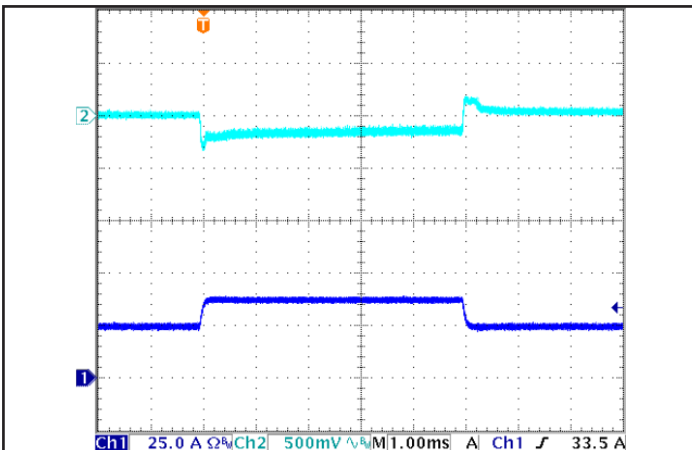
Figure 9: Output voltage response to step-change in load current [50%-75%-50% of I_{out(max)} ; dI/dt = 0.1A/\mu s ]. Load cap: 1\mu F ceramic and 470\mu F , 15mW ESR electrolytic capacitors. Top trace: Vout (500mV/div), Bottom trace: Iout (25A/div).
